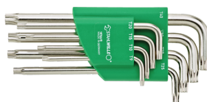
96432200 TORX® L-Key set
